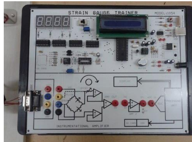
Strain Gauge Trainer
