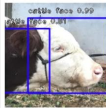
(a) RetinaNet
